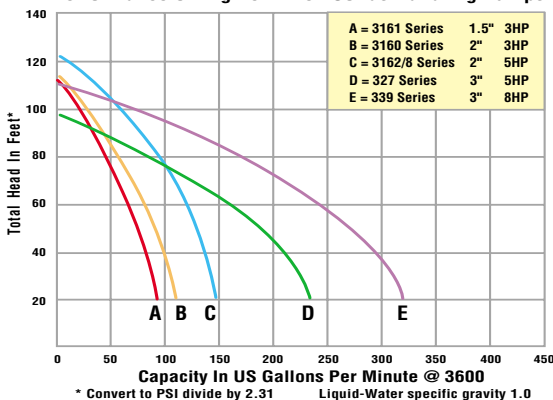
Performance of Engine Driven Solids Handling Pumps
