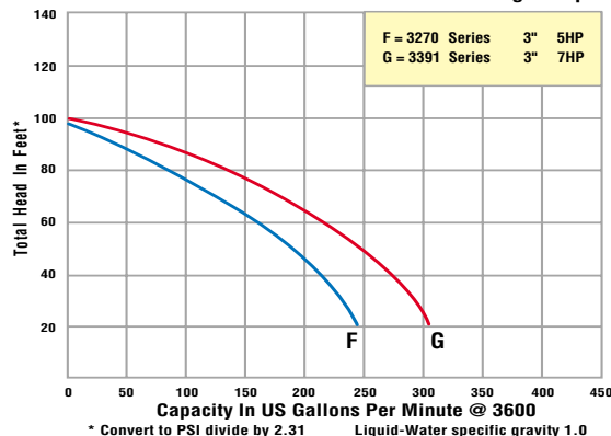
Performance of Diesel Driven Solids Handling Pumps
